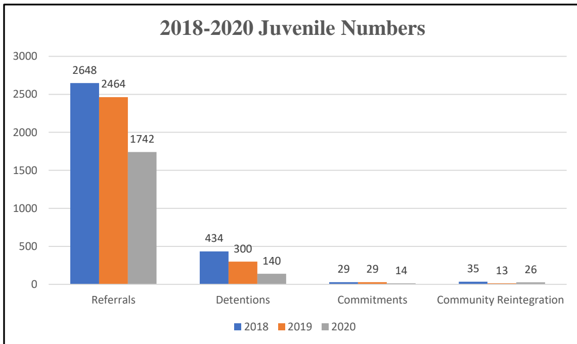
Figure 2: 2018-2020 Juvenile Numbers
